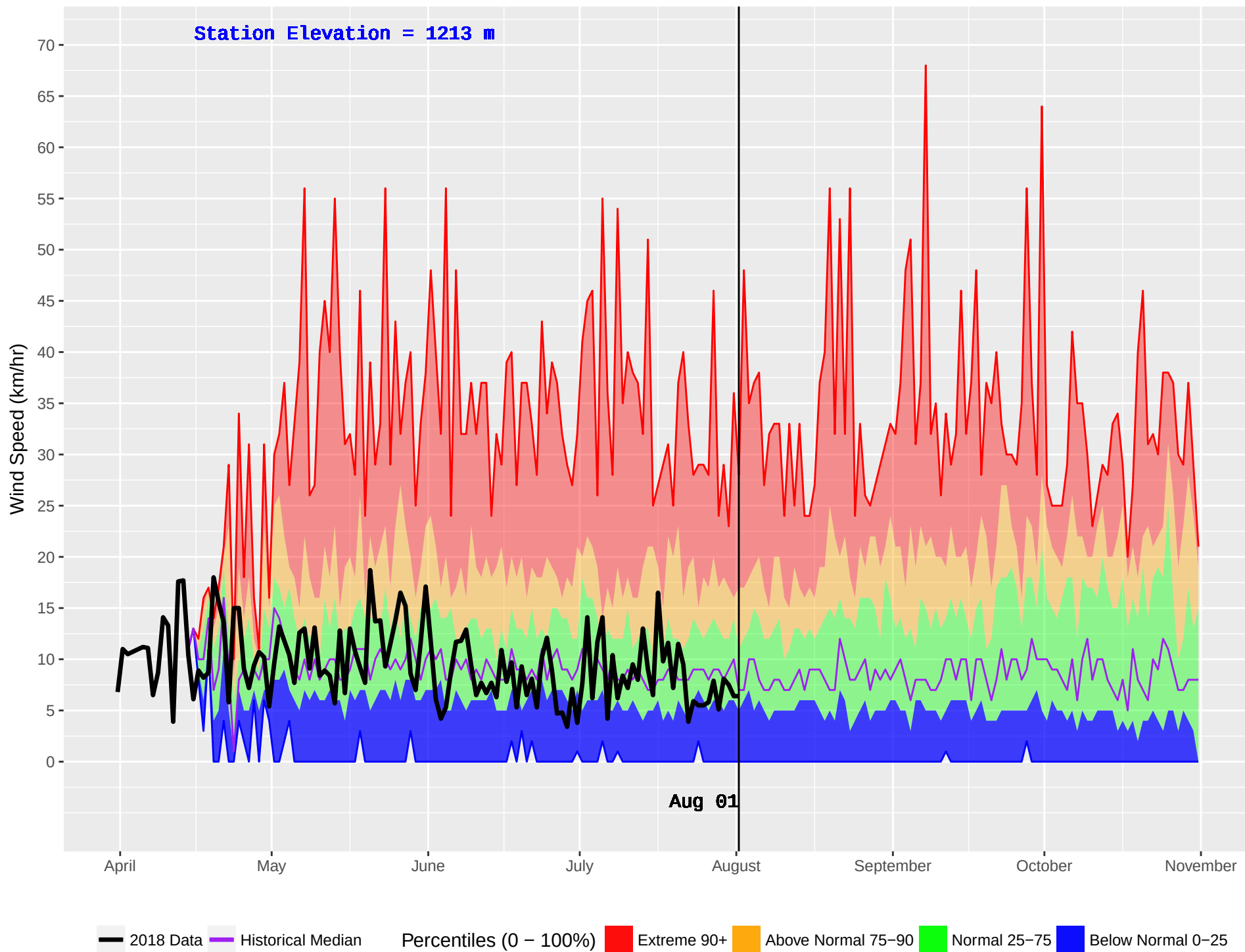
INGENIKA POINT (145) : Historical (1971–2016) and Current (2018) Daily Wind Speed
